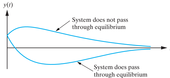
Figure 8.5.6: Critical damping: The system can pass through equilibrium at most once.
