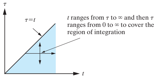
Figure 10.9.1: Changing the order of integration in Theorem 10.9.3.
